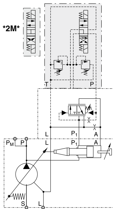
Schematics PVAC2M*/PVAC2E*
