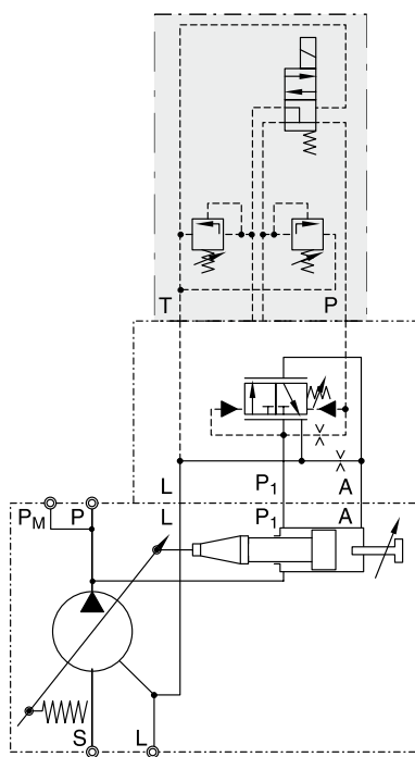
Schematics PVAC2P*
