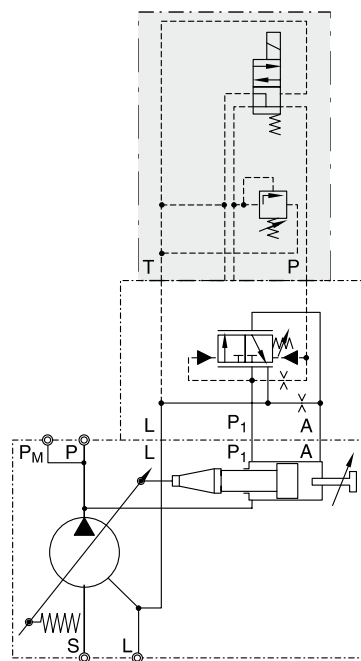
Schematics PVAC1E*
